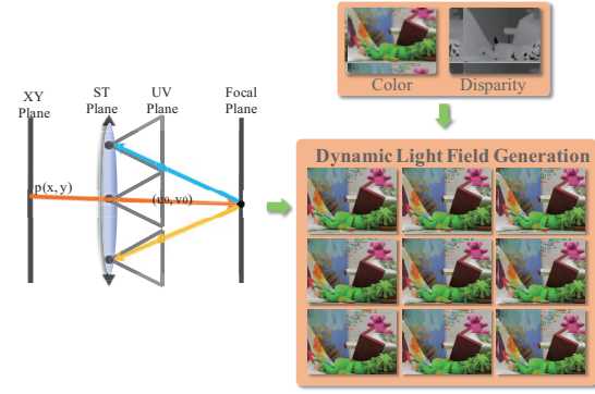
Fig. 8 We synthesize an in-lens light field (left) from the recovered high-resolution color image and disparity map (right).
