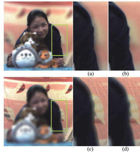
Fig. 7 Comparing results generated by image space blurring (a, c) and our light field synthesis method (b, d). Our approach effectively reduces both the intensity leakage (a) and boundary discontinuity (c) artifacts.
