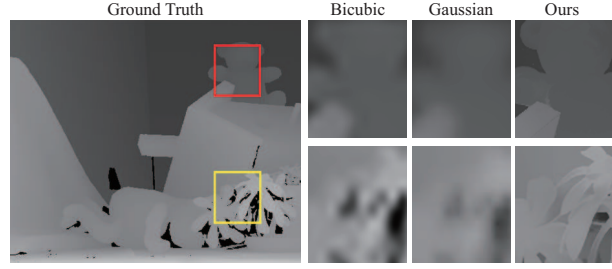
Fig. 5 Comparison of our method and other upsampling schemes on synthesize data. Both patches in the disparity map are upsampled from a resolution of 30 \times 25 to 450 \times 375 .
