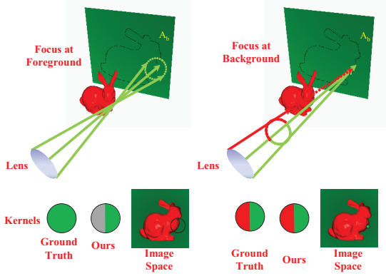
Fig. 9 Illustrations of two types of boundary artifacts. See Section 4.3 for details.
